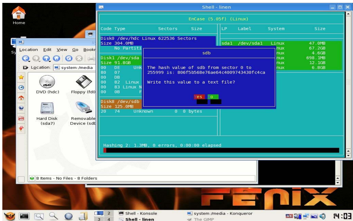
Figure 24: Linen in FENIX showing hash value of /dev/sdb (pre-mount)
