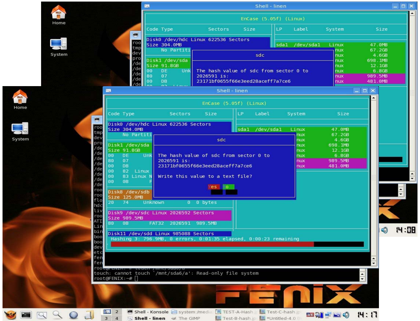
Figure 38: Linen tests hash values both pre-mount and post-mount to determine if mounting changes hash
