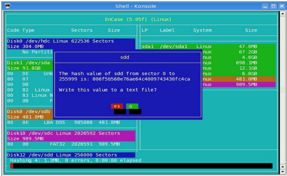
Figure 37: After reboot, names of devices are changed, /dev/sdb is moved to /dev/sdd but hash value remains unchanged
