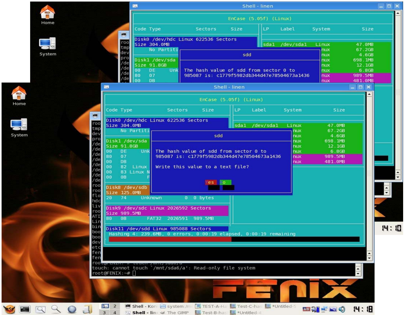
Figure 43: Hashes before and after mounting the device, notice the times
